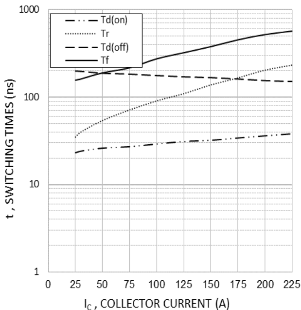
Fig. 7 Typical switching times as a function of collector current (inductive load, T_{yj}=25^{\circ}C , V_{CE}=400V , V_{GE}=15/0V , r_G=8\Omega )
