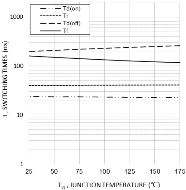
Fig. 9 Typical switching times as a function of junction temperature (inductive load, V_{CE}=400V , V_{GE}=15/0V , I_C=30A , r_G=8\Omega )
