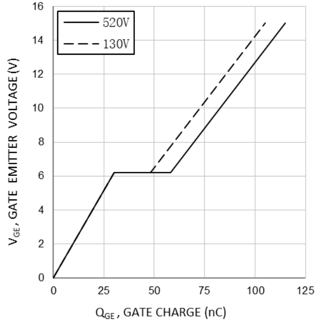
Fig. 14 Typical gate charge ( I_c=30A )
