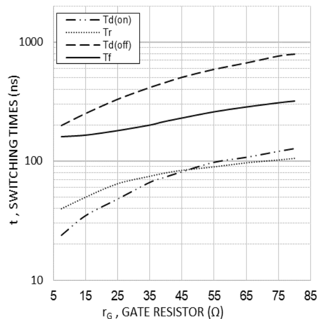
Fig. 8 Typical switching times as a function of gate resistance (inductive load, T_{yj}=25^{\circ}C , V_{CE}=400V , V_{GE}=15/0V , I_C=30A )
